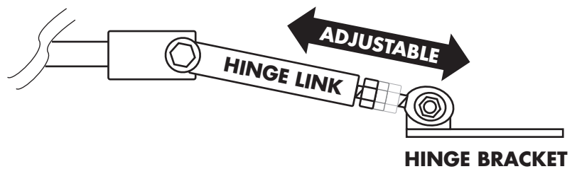
Diagram C - Closeup Hinge Link Fine Tuning
