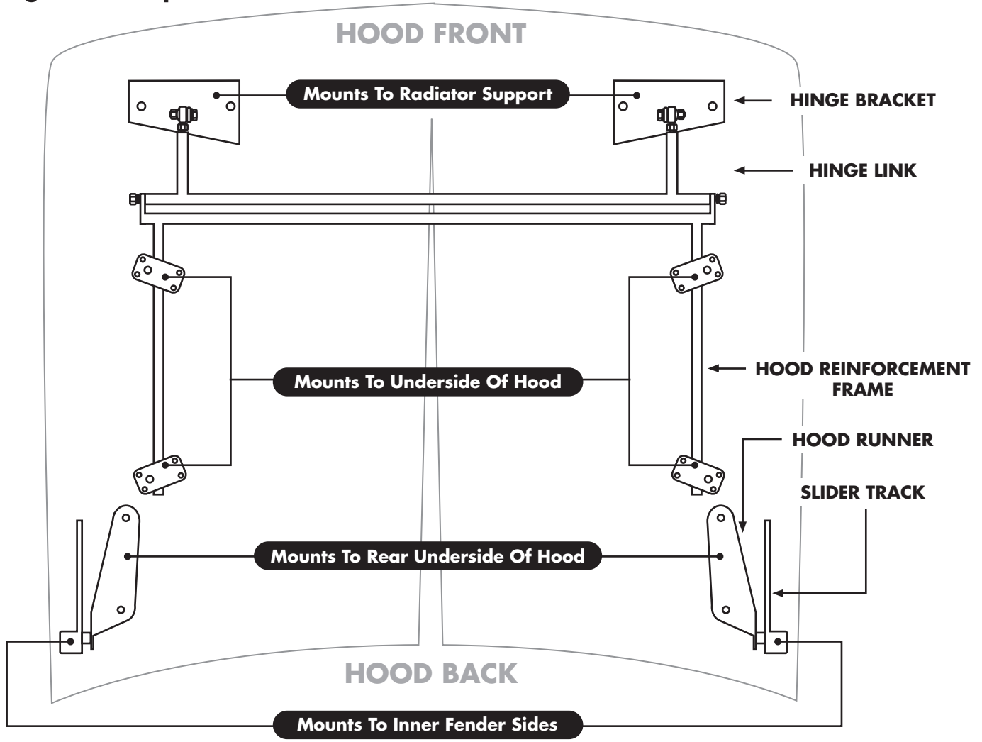
Diagram A - Top View of Hood
